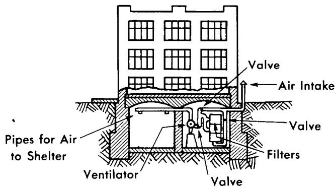
VENTILATING SYSTEM
